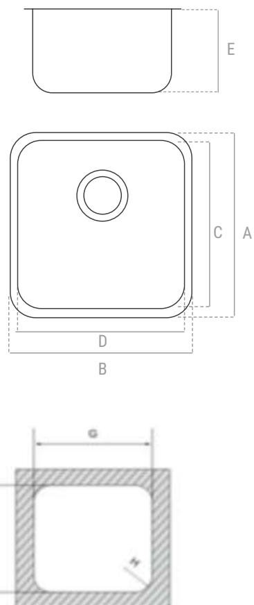
MEDIDAS ENCASTRE | DIMENSIONS ENCASTREMENT | INSTALL DIMENSIONS
